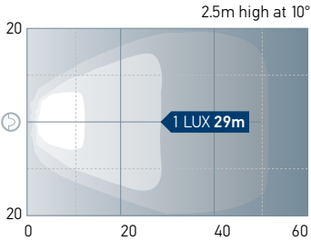
Beam Pattern Dual Colour-Spread
