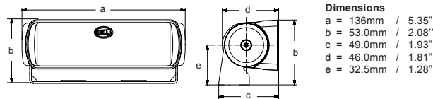
Sea Hawk R Recessed Mount
