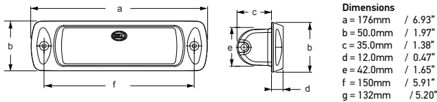
Sea Hawk R Recessed Mount
