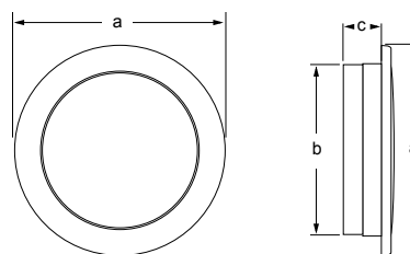
Dimensions a = 150 mm / 5.90" b = 124 mm / 4.88" c = 20 mm / 0.79"
