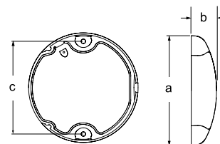
Dimensions a = 129.5mm / 5.10" b = 29.5mm / 1.16" c = 110mm / 4.33"
